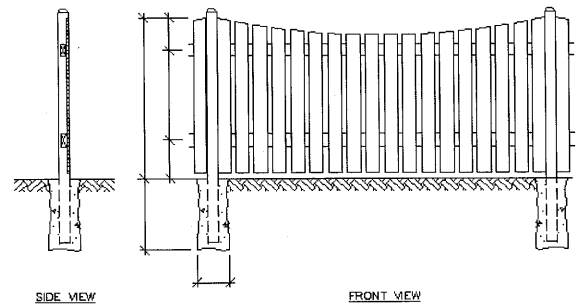
4' SCALLOPED SPACED PICKET FENCE DETAIL STYLE : TOE NAIL NOTES:
